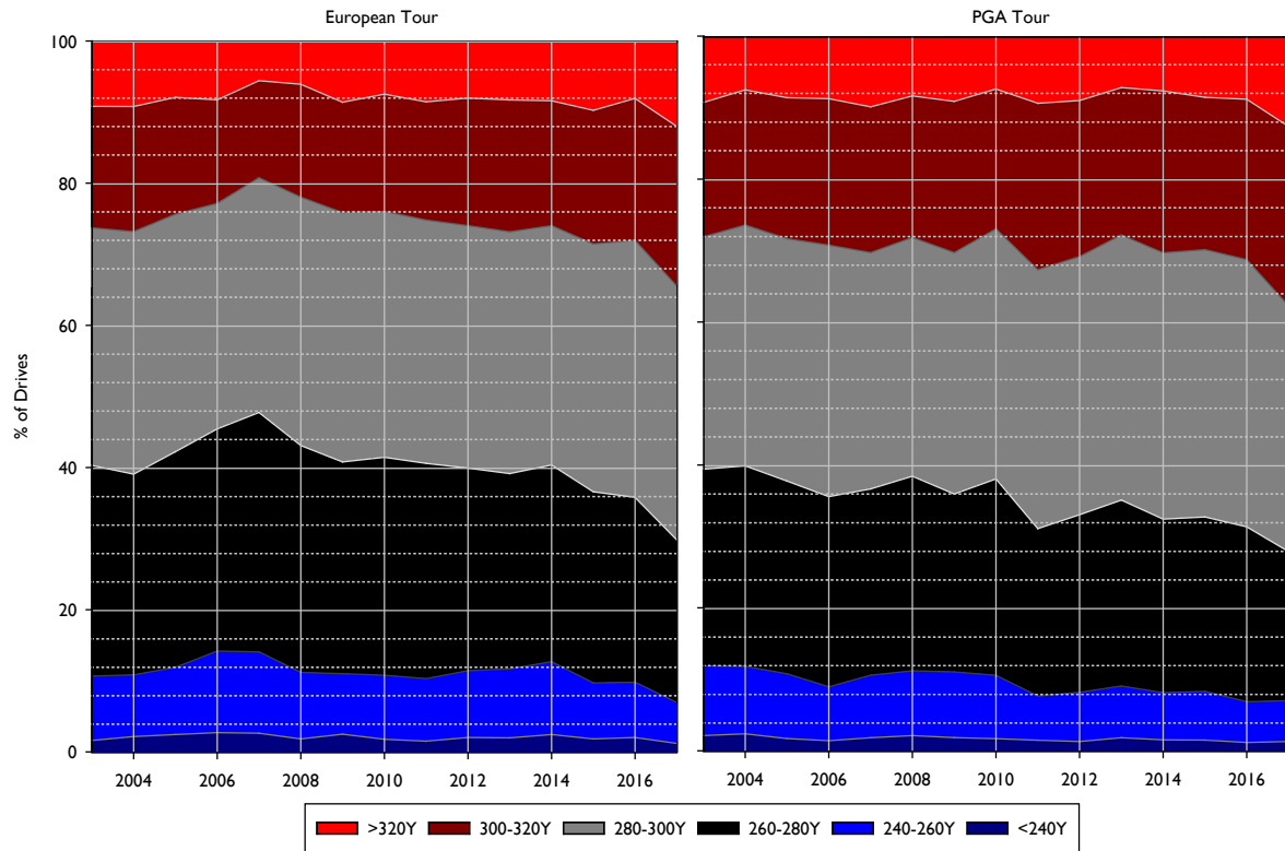
Figure 10. The distribution of drives on “measured” driving holes on the European and PGA tours 2003-2017.
